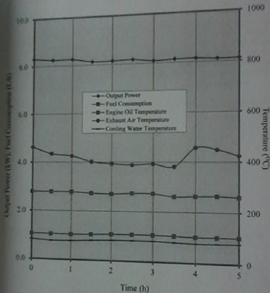
Figure 4. Performance characteristic curves during the continuous running test of the GOLDEN BOW JG 140DI diesel engine
