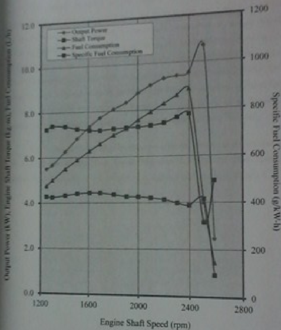
Figure 3. Performance characteristic curves of the GOLDEN BOW JG 140DI Diesel Engine
